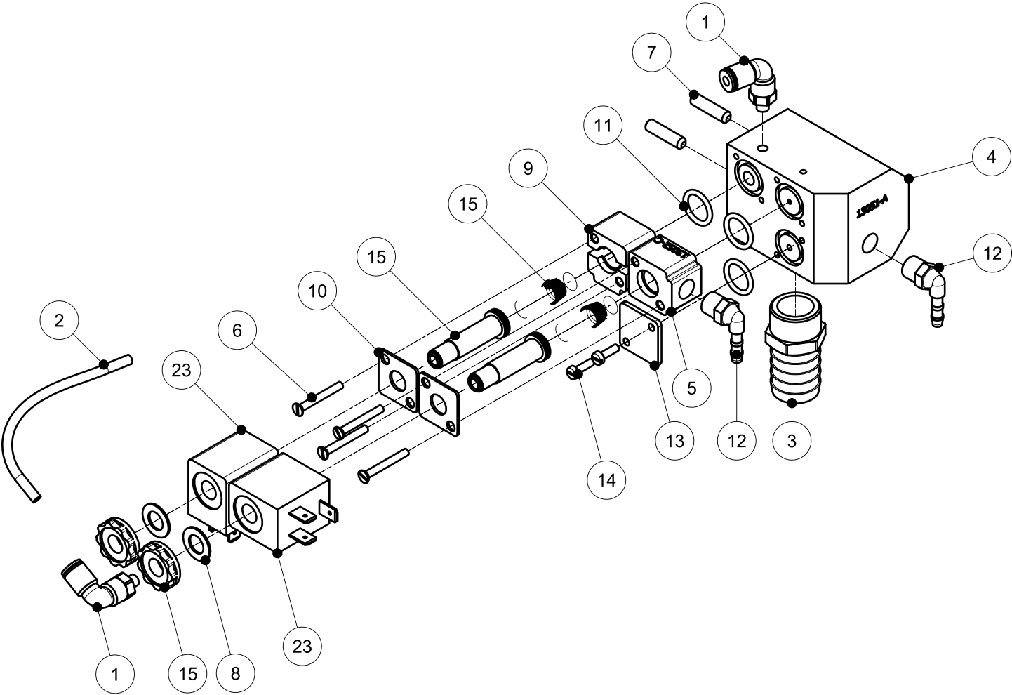
Air Valve
