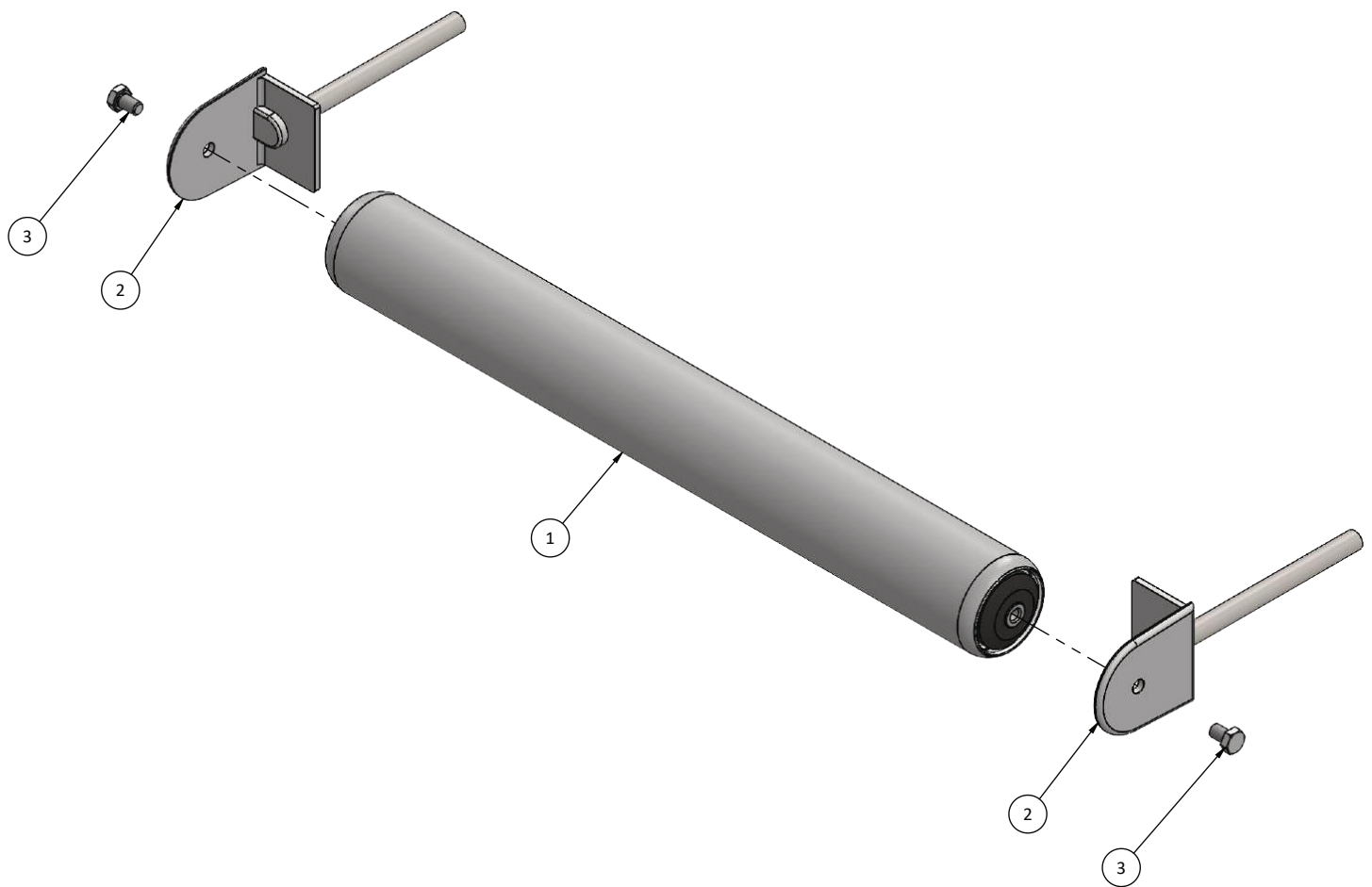
Belt Roller
