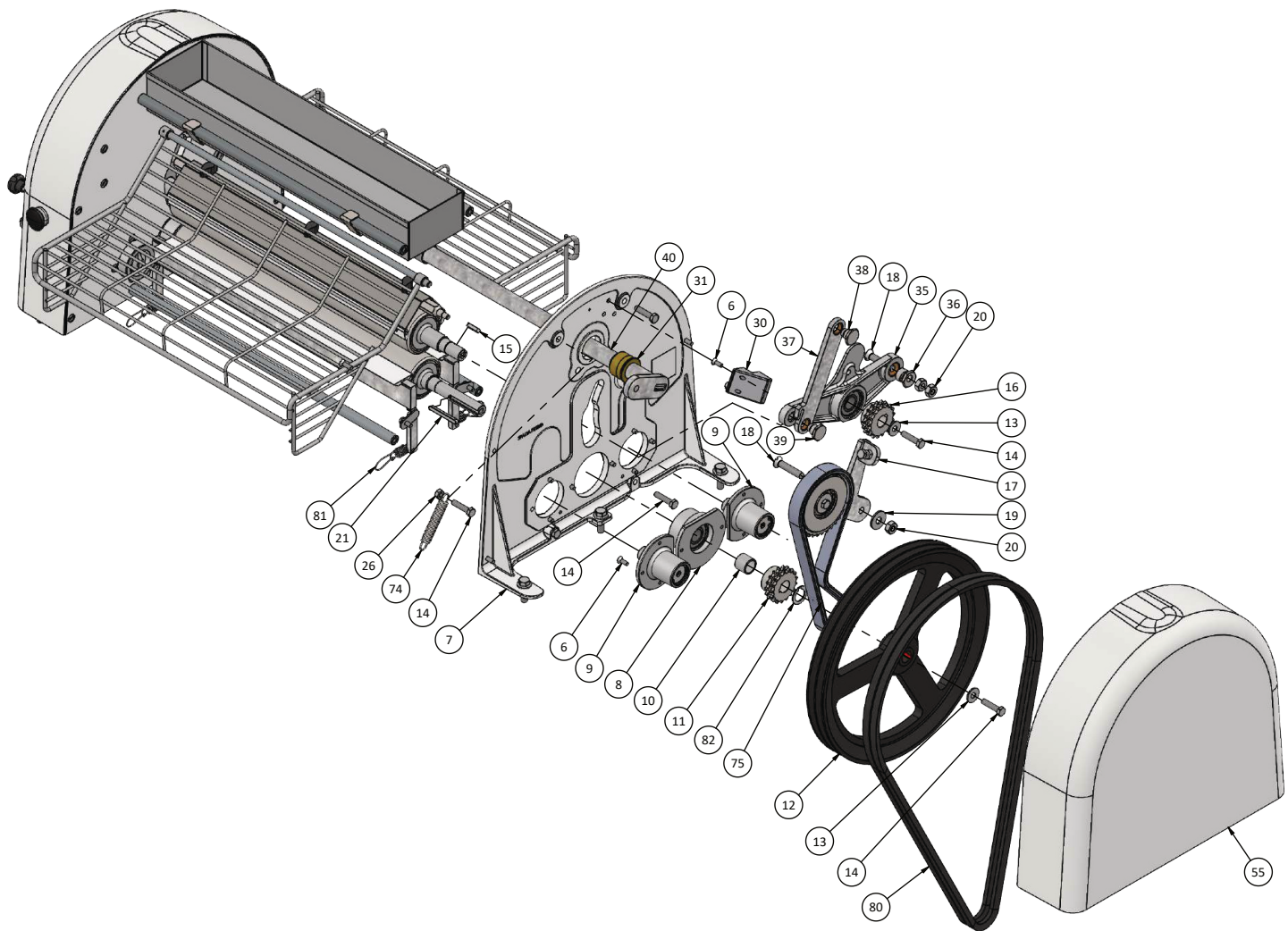
Roller Assembly
