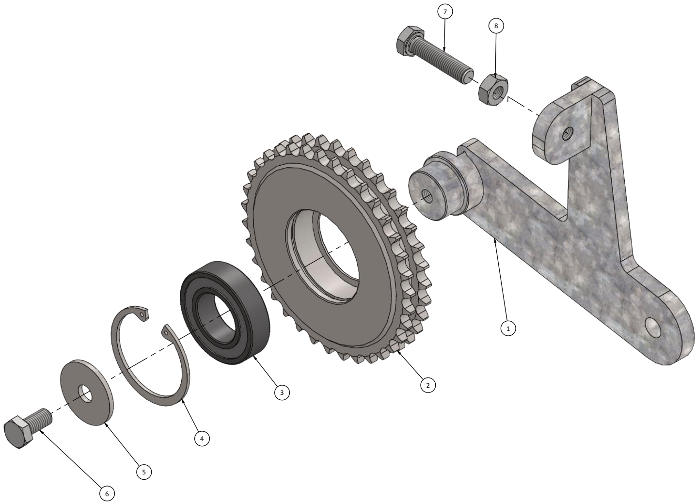
Chain Tensioner
