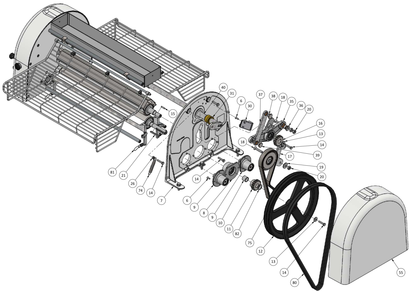
Roller Assembly
