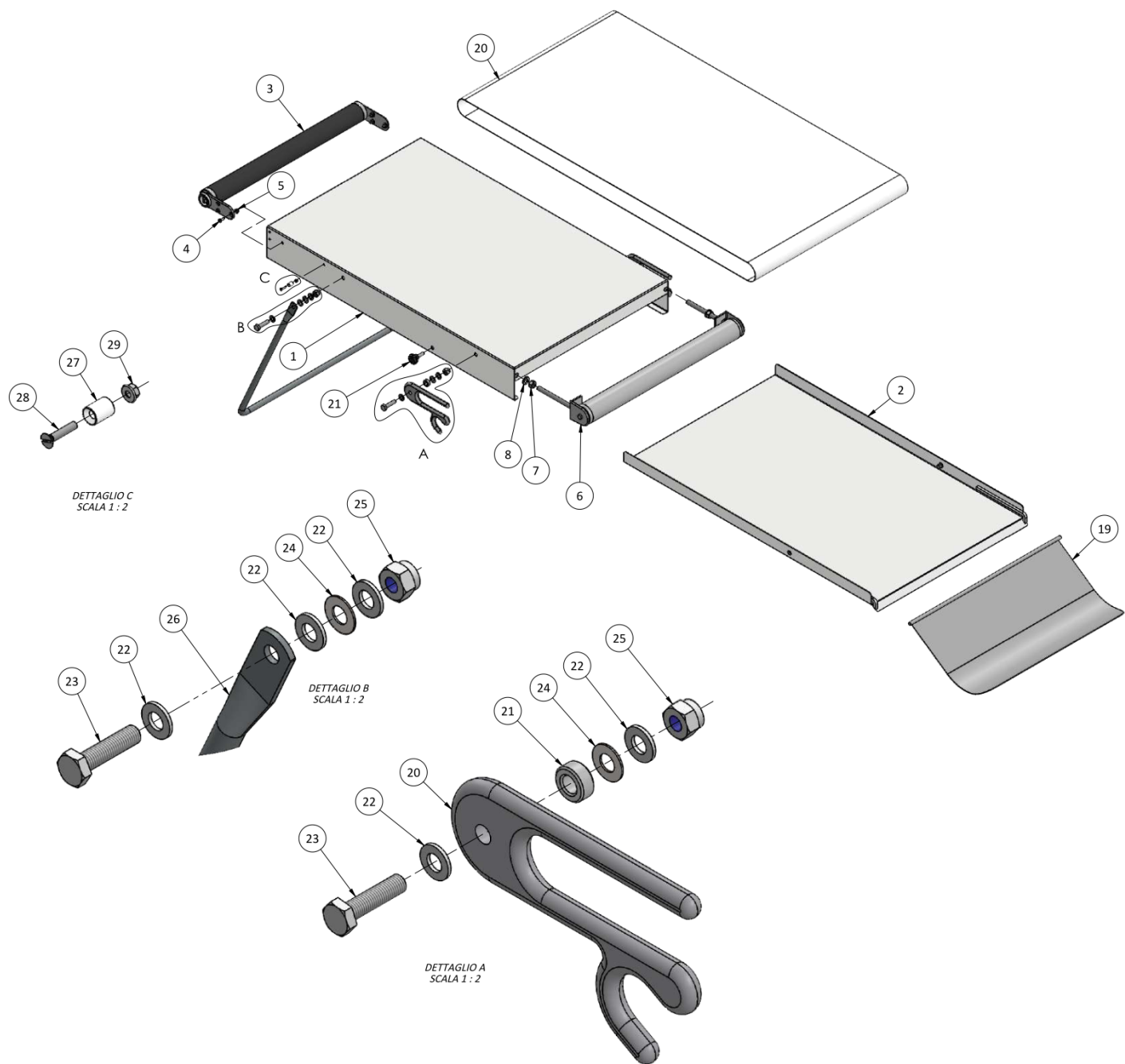
Right Table Assembly
