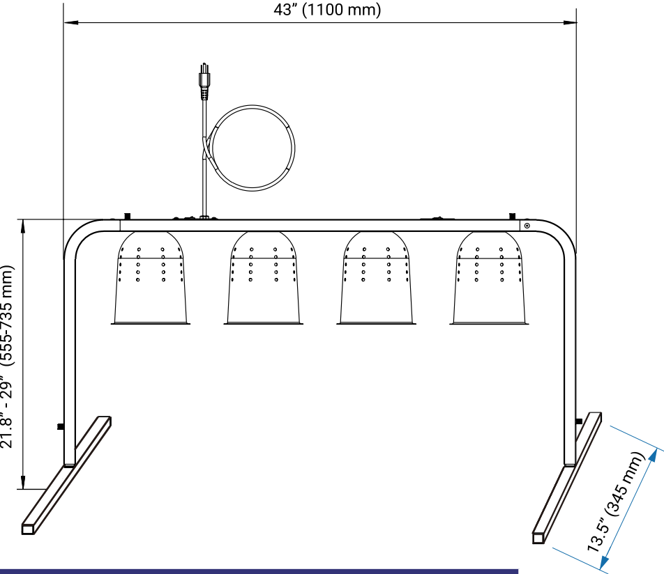
TECHNICAL DRAWING (48396)
