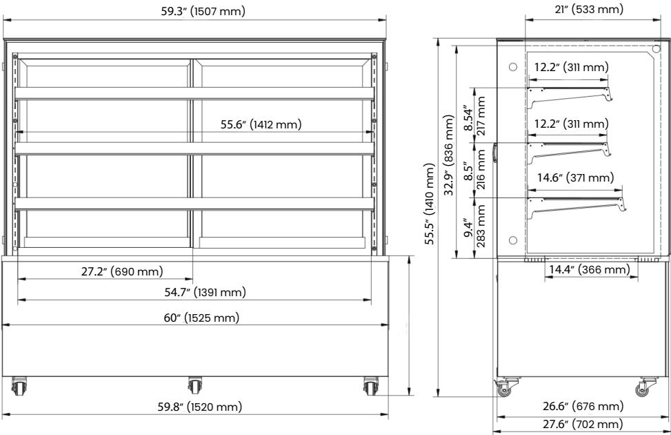
Item 44384 Technical Drawings Unit of Measurement: inch / mm
