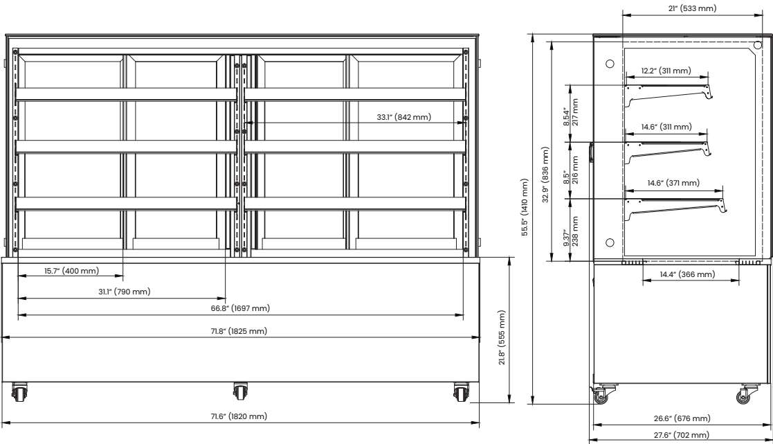
Item 44505 Technical Drawings Unit of Measurement: inch / mm
