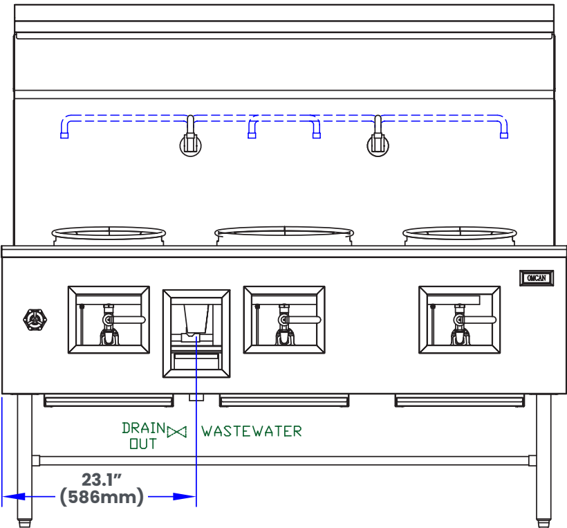
TECHNICAL DRAWING (48409)
