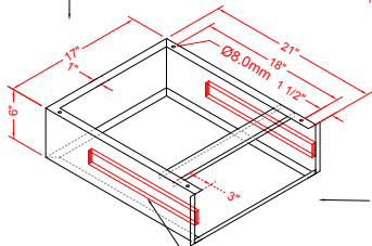
Connecting Rail
