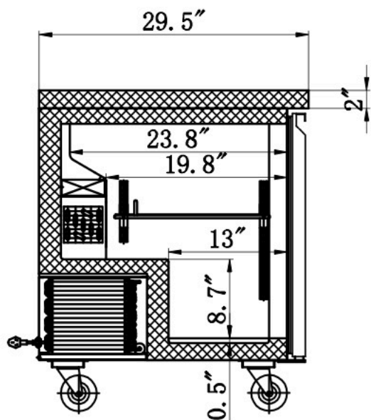
SECTION VIEW
