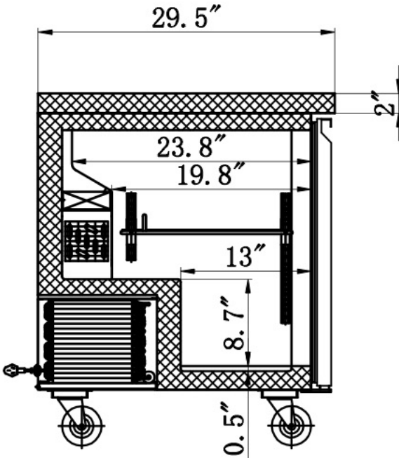
SECTION VIEW
