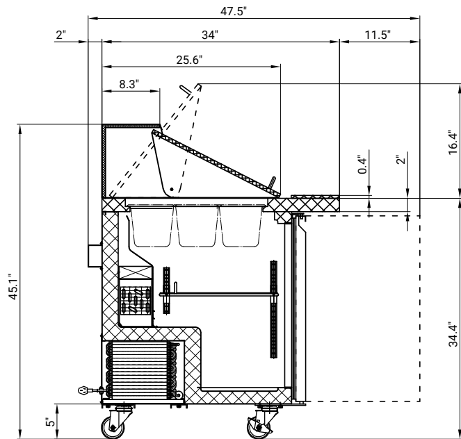
SECTION VIEW
