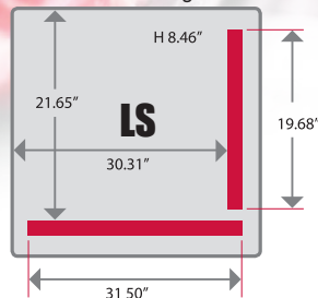
VP-NL-0063-M Configuration
