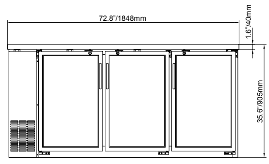
73-inch 3 doors bottle cooler Item: 37549 Model: BB-CN-0020-S
