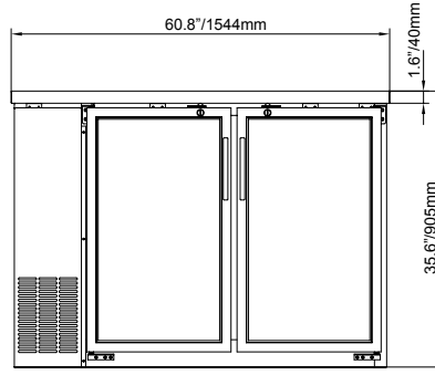
61-inch 2 doors bottle cooler Item: 37548 Model: BB-CN-0016-S
