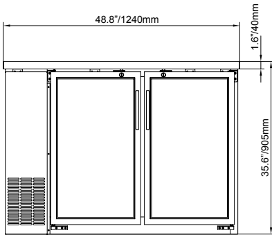
49-inch 2 doors bottle cooler Item: 37547 Model: BB-CN-0012-S
