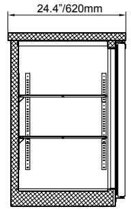
73-inch 3 doors bottle cooler Item: 37549 Model: BB-CN-0020-S
