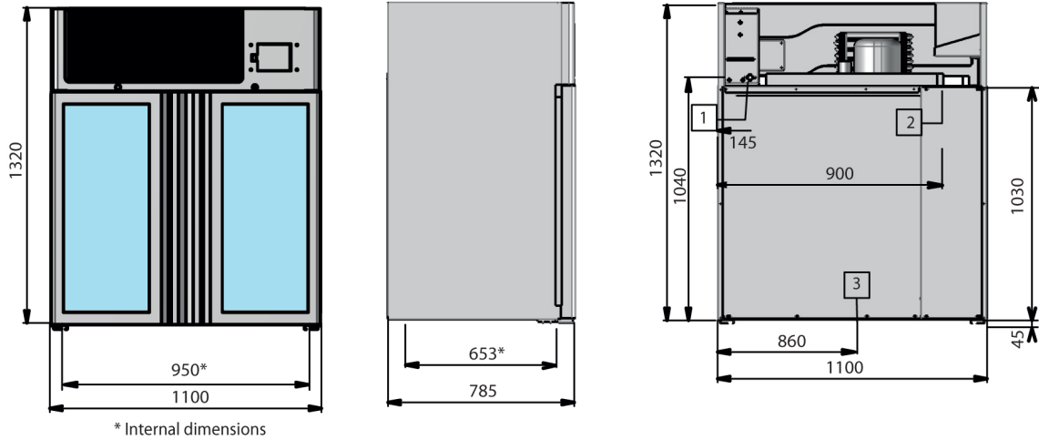
1. Water inlet: 3/4" Dia. 2. Electrical connection: 230V 3. Water outlet: 1/2" Dia. *Internal dimensions
