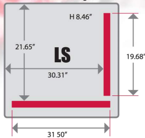
VP-NL-0063-M Configuration
